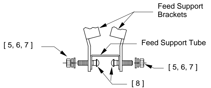
DETAIL B
