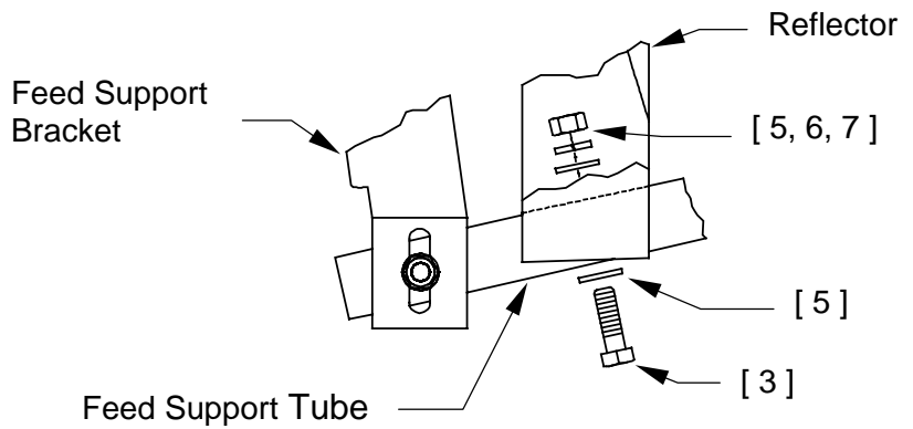
DETAIL D
