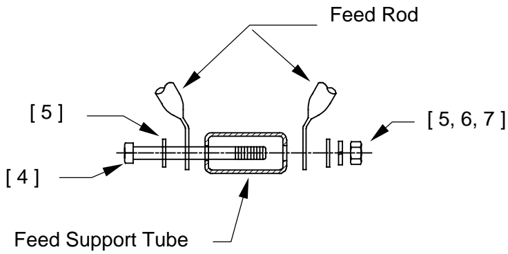
DETAIL C
